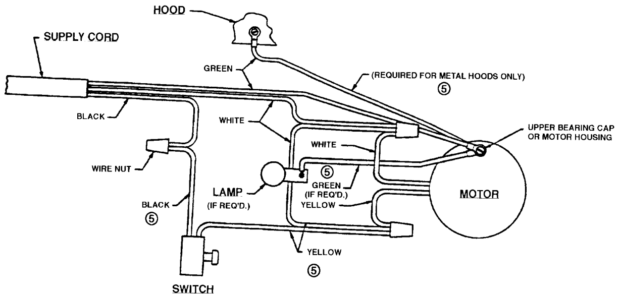
36575 WIRING DIAGRAM
